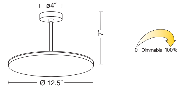
9911/4*LED
